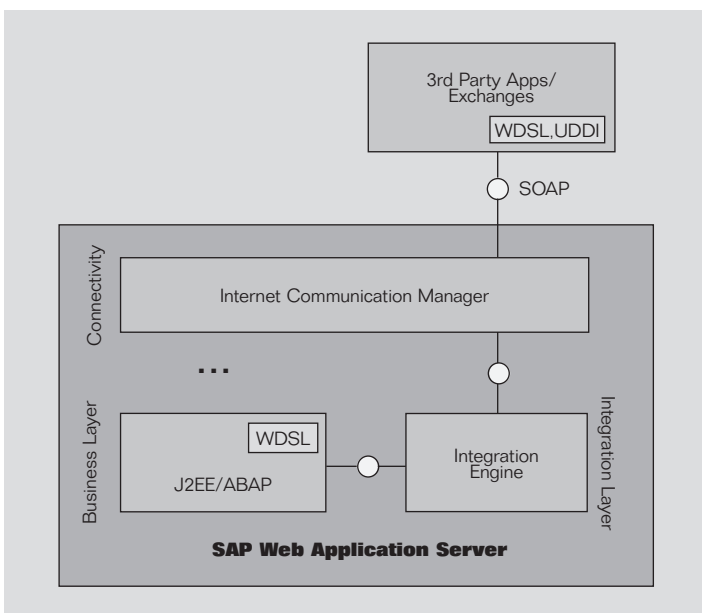
Figure 2: Provision of Web services
